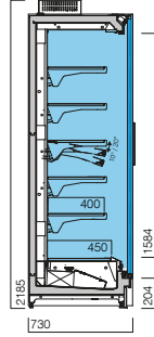
MF2 700 P CP SG 3M1/3M2 carne, charcutaria laticínios meat, delicatessen dairy products
