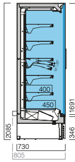
MF2 700 P CP CG 3M1/3M2 carne, charcutaria laticínios meat, delicatessen dairy products
