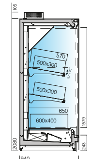
MF2 900 PF CC SG 3H1 frutas, legumes e flores produce and flowers
