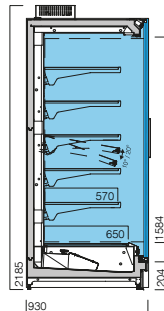
MF2 900 P CP SG 3M1/3M2 carne, charcutaria laticínios meat, delicatessen dairy products
