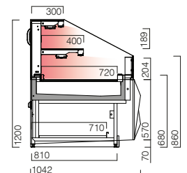
SMDSAQ - VSF semimural aquecido multidesk display heated semi murale chauffé semi mural calentado
